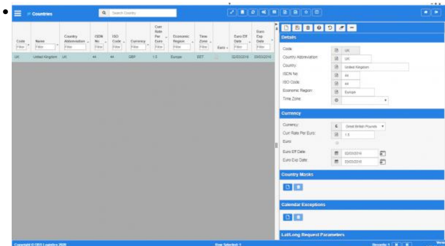
Countries maintenance
