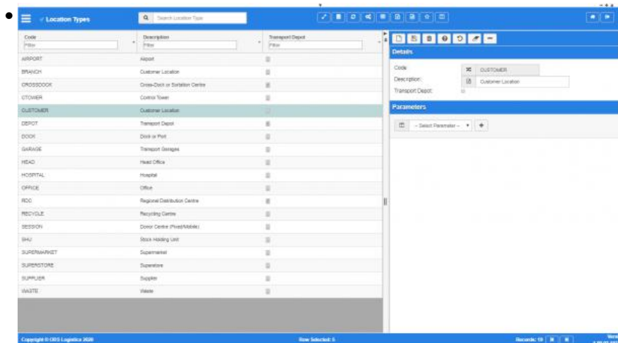
Location types
