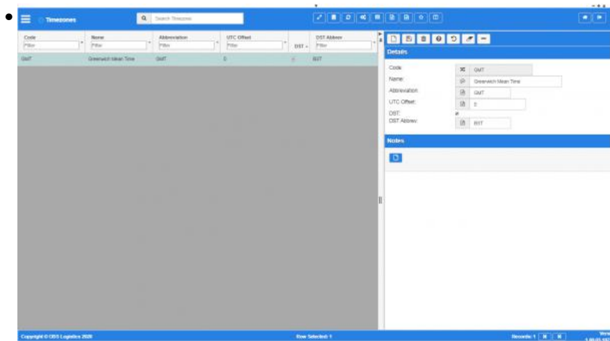
Timezones maintenance
