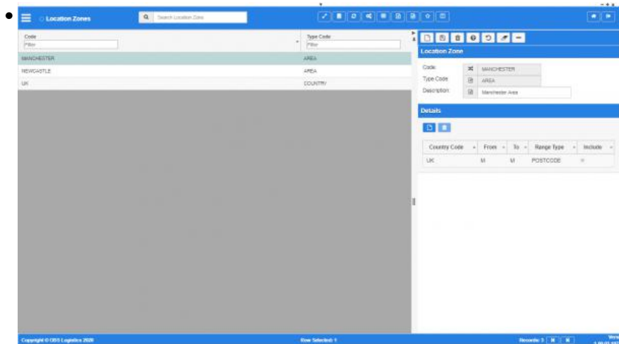
Location zones
